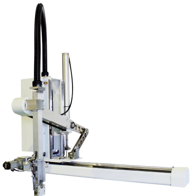
The new SWA-3K-R5 model with 3-kg useful load, for the extraction of moulded components
