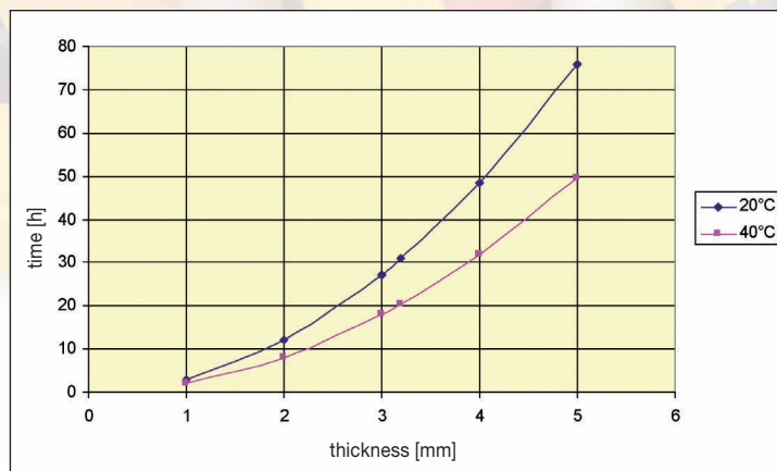
Fig. 2 - 2% absorption in water at 20°C and 40°C
