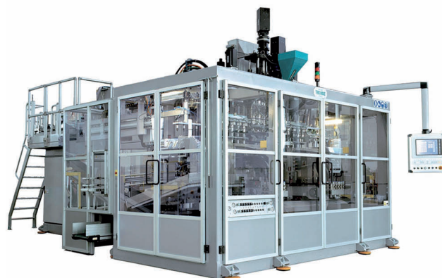
The double shuttle machine exhibited by Techne is dedicated to the -production of 200-ml round bottles for drinkable yogurt, neck to neck, 40 cavities, for a total production capacity of 12,000 bottles per hour
