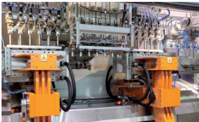
The extrusion head of the PB10E/DXL blow moulding machine has been designed to allow a greater control of the extruded parison and permits color changes in less than half an hour
